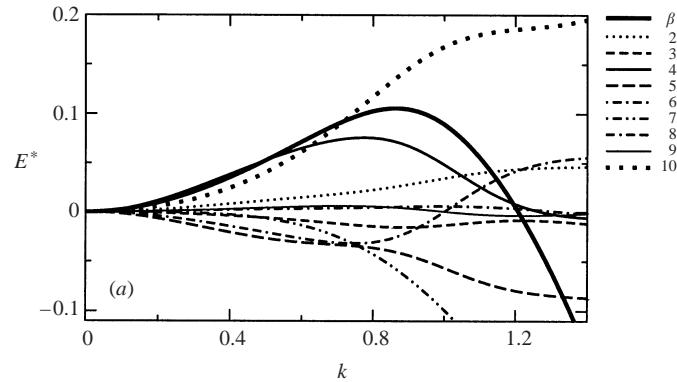
FIGURE 12. The contributions to the largest eigenvalue of the various terms of the operator relative to their contributions to the marginally stable state at k = 0 plotted as a function of the wavenumber with Ma^* = 5.0 , Bo^* = 4 , Bi = 0.12 and l/L = 20 .
